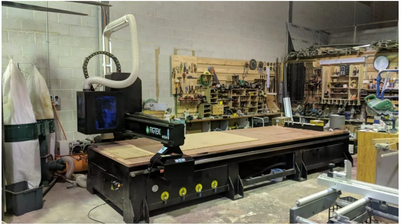
Example of Large Scale Industrial size CNC Router. Circa $33,000
